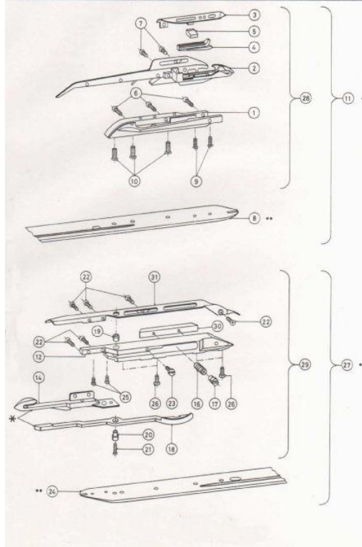
SINGLE PARTS OF GRIPPER MBJ2
