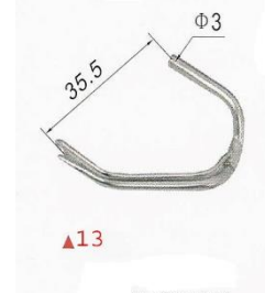
NVC2.1/150 A13 NEEDLE 35,5 MM DIAM 3 MM
