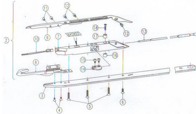
SINGLE PARTS OF MBJ3 GRIPPER RHS
