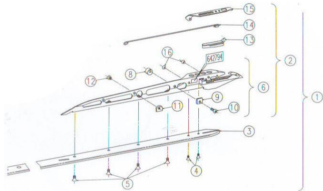
SINGLE PARTS OF MBJ3 GRIPPER LHS
